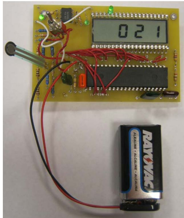
b) Soldered PCB for force sensor
