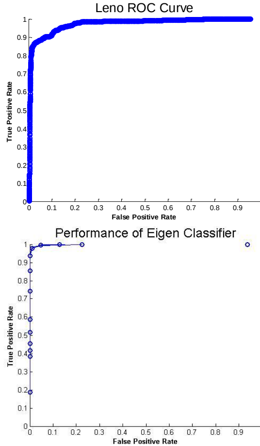
Figure 2: ROC Curves of Both Approaches
